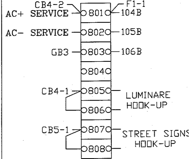
B.B.U. INTERFACE INSIDE INTERSECTION CABINET
