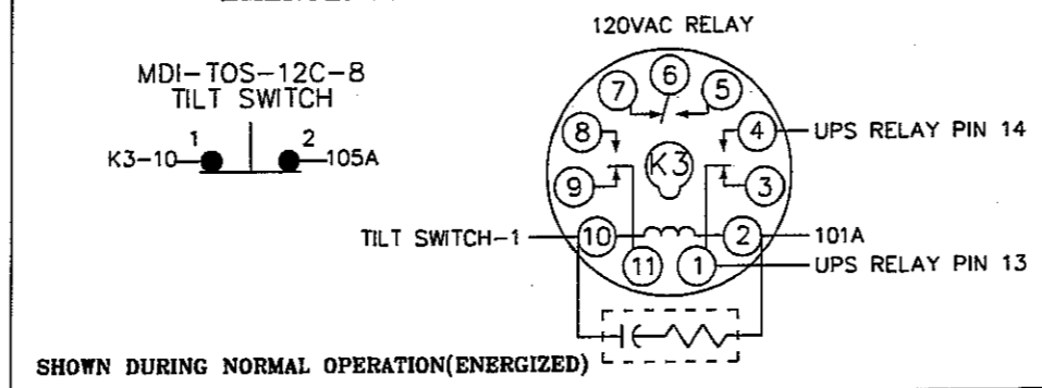
EMERGENCY POWER OFF CIRCUIT
